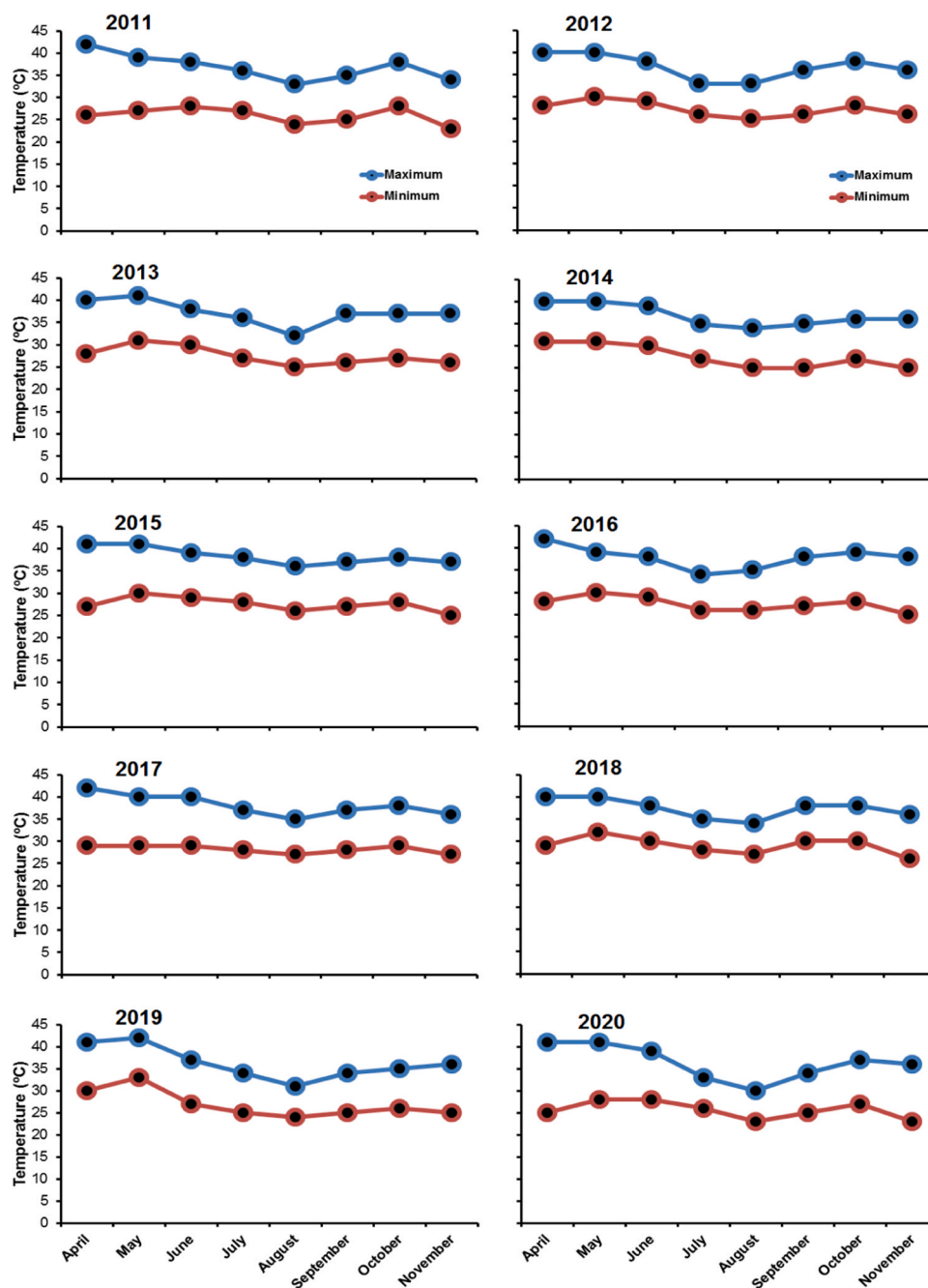
Fig. 3. Average monthly maximum and minimum temperature for disturbed and undisturbed sites in DBR for ten years (2011–2020), calculated based the data obtained from SMA.
